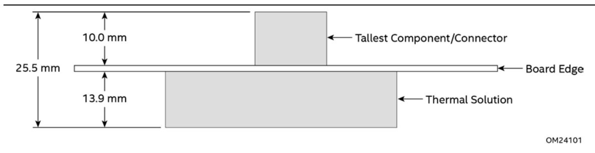
Figure 17. Board Height Dimensions
